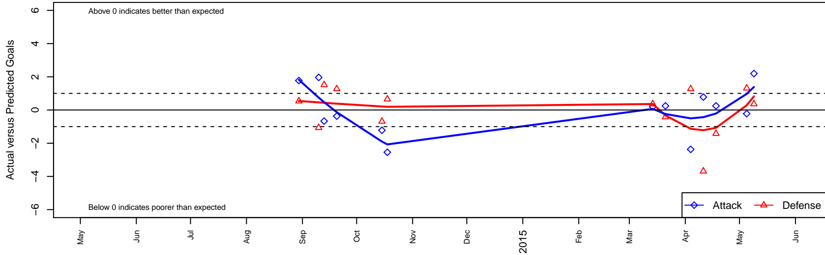
Boise Nationals SC Breakers White G03 Dots are actual minus expected GF (blue circles) and GA (red triangles). Blue line is smoothed change in attack strength. Red is smoothed change in defense strength.
